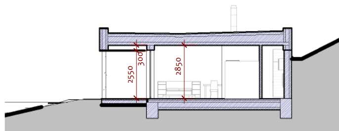
3 1:200 REZ B
